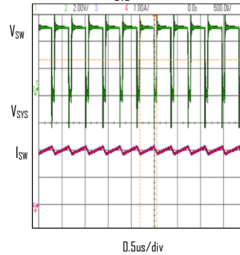
DCDC PWM SWITCHING WAVEFORM I sys =2A
